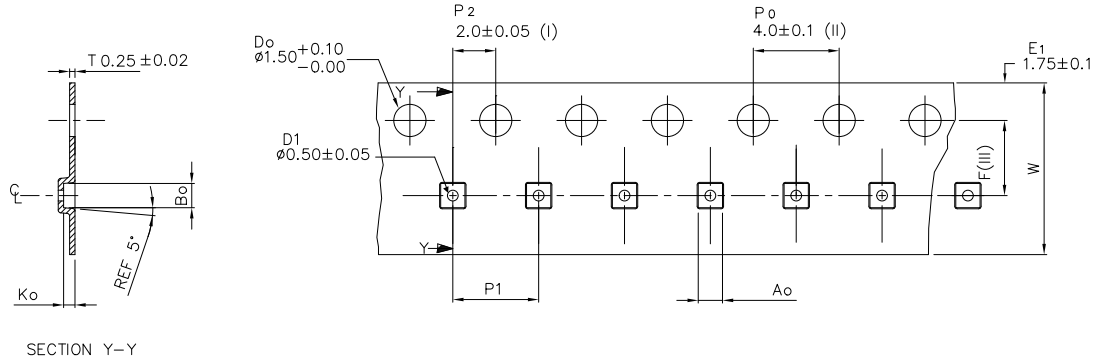
Figure 24. Tape dimensions
