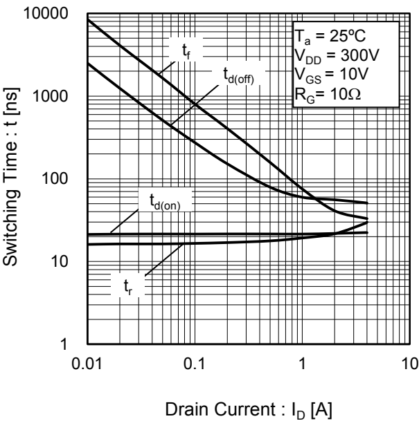
Fig.18 Switching Characteristics
