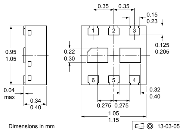
Fig. 12. Package outline DFN1010B-6 (SOT1216)
