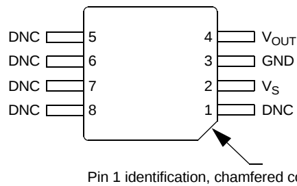
Figure 2. Device pinout (top view)
