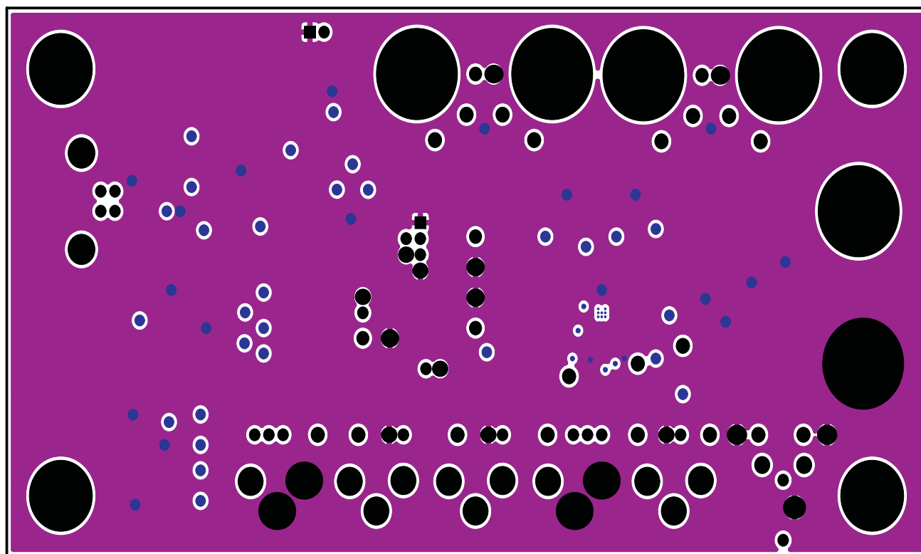
Figure 9. TPA2054D4EVM – Layer 2
