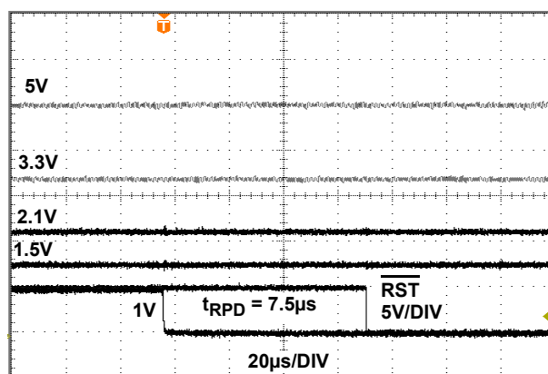
FIGURE 6. ISL88031 t_{RPD}
