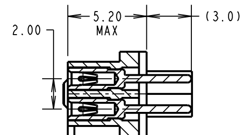
SECTION X-X
