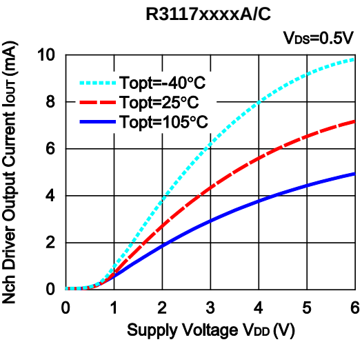
6) Nch Driver Output Current vs. Supply Voltage 7) Nch Driver Output Current vs. V DS
