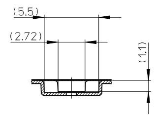
SECTION X-X
