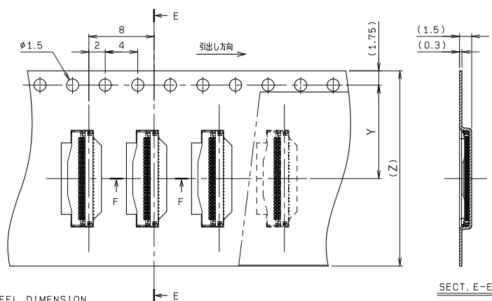
REEL DIMENSION
