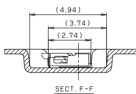
SECT. F-F
