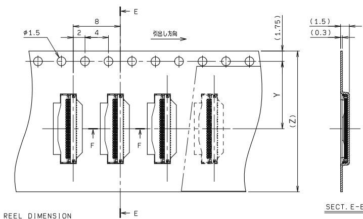
REEL DIMENSION
