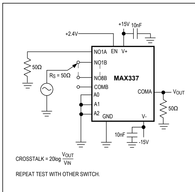
Figure 7. Crosstalk
