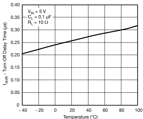
Figure 23 - SiP32416 Turn-Off Delay Time vs. Temperature
