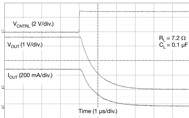
Figure 25 - SiP32413 Channel 1 Turn-Off ( V_{IN} = 3.6 V, R_L = 7.2 Ω)
