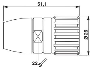
Dimensional drawing
