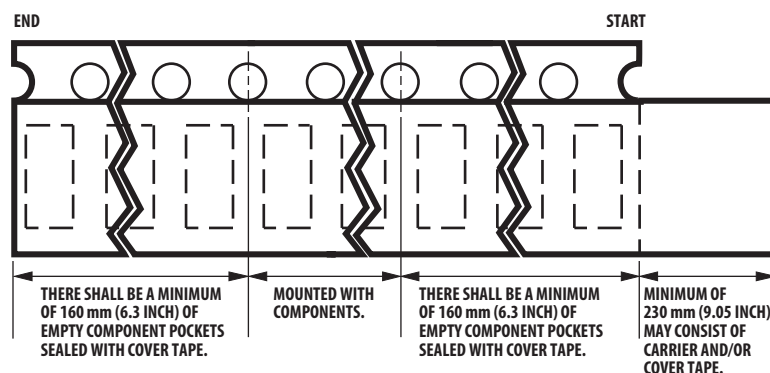
Figure 11. Tape dimensions.
