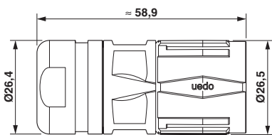
Dimensional drawing
