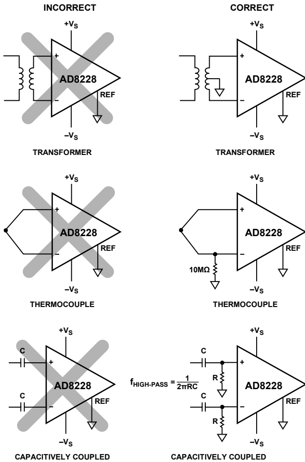
Figure 46. Creating an IBIAS Path
