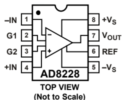
Figure 44. Pinout Diagram
