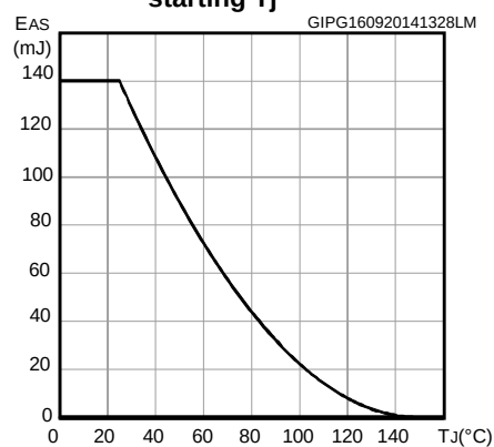
Figure 17: Maximum avalanche energy vs starting T_J
