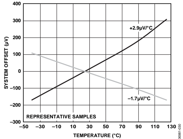
Figure 7. System Offset vs. Temperature, Normalized at 25^\circ\text{C} , Referred to Output
