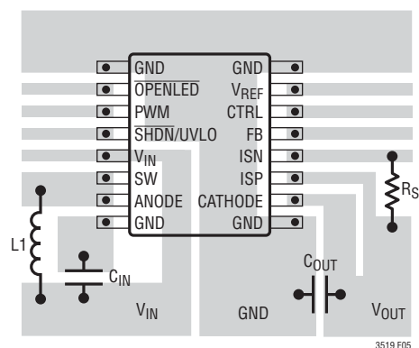
Figure 5. Suggested Layout
