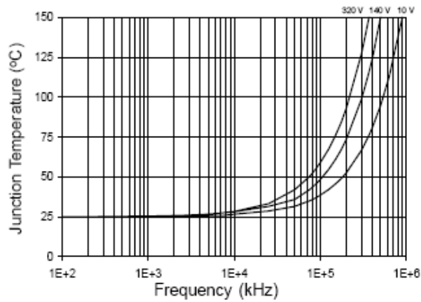
Figure 35. IRS2110S/IRS2113S T_J vs. Frequency (IRFPE50) R_{GATE} = 10 \Omega , V_{CC} = 15 \text{ V}
