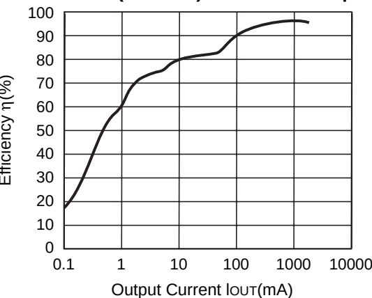
R1224N502E ( V_{IN}=6.5V ) CDRH127-10 \mu H
