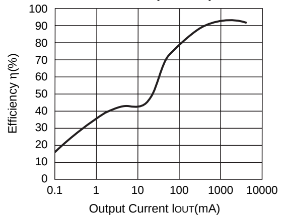
R1224N502G ( V_{IN}=10V )
