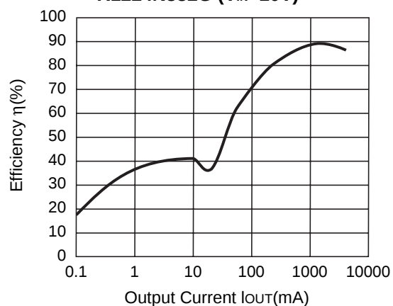
R1224N332G ( V_{IN}=10V )
