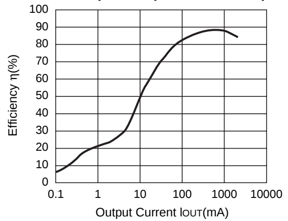
R1224N182M ( V_{IN}=5.0V ) CDRH127-27 \mu H
