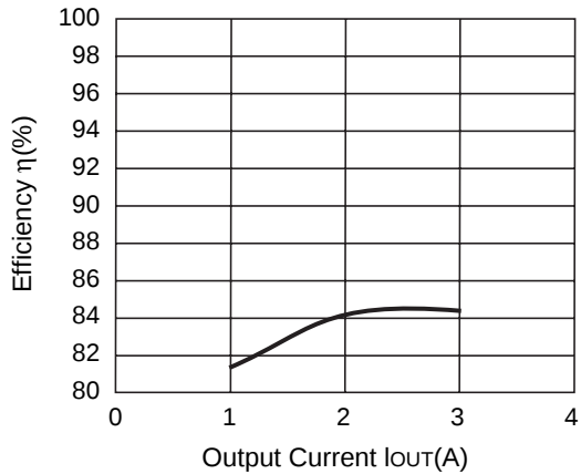
R1224N332M ( V_{IN}=18V )
