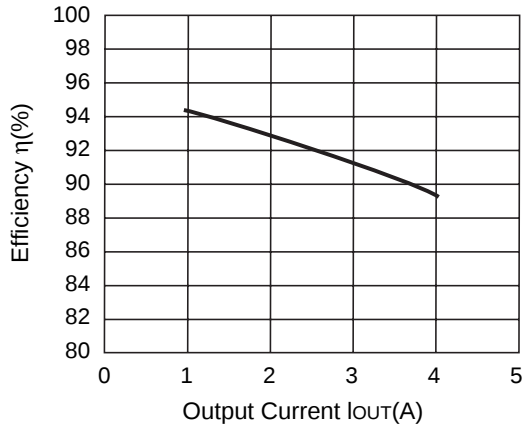
R1224N332M ( V_{IN}=5V )
