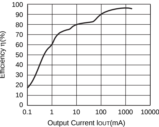
R1224N502E ( V_{IN}=6.5V ) CDRH127-10 \mu H
