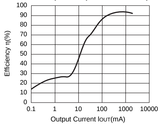
R1224N332H ( V_{IN}=4.8V ) CDRH127-10 \mu H
