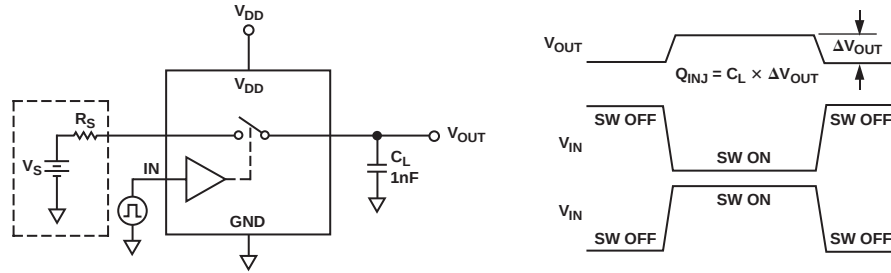
Test Circuit 7. Charge Injection
