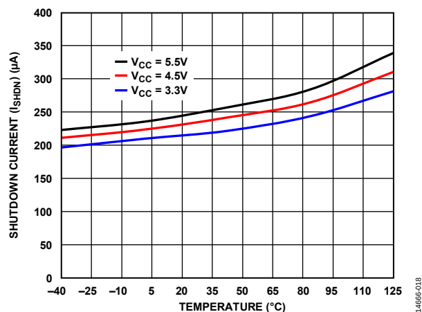
Figure 15. Shutdown Current ( I_{SHDN} ) vs. Temperature
