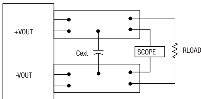
Figure 5. Measuring Output Ripple and Noise (PARD)
