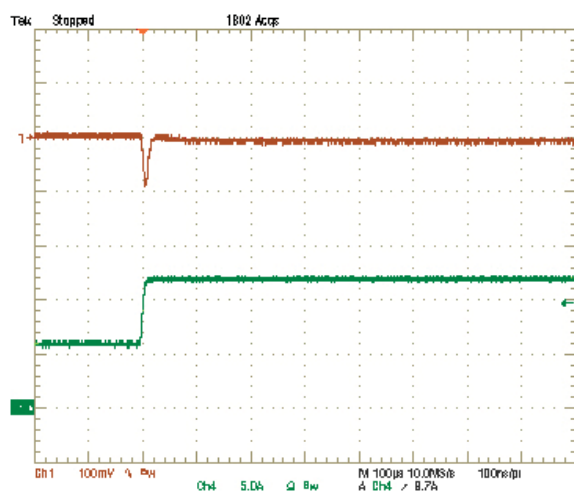
Step Load Transient Response (Vin=5V, Vout=0.6V, Cload=94μF, Iout=6A to 12A) Trace 1=Vout, 100 mV/div, Trace 4=Iout, 5A/div.
