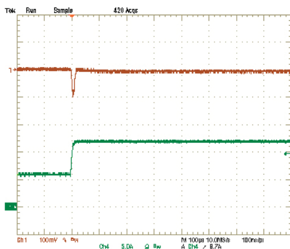
Step Load Transient Response (Vin=5.0V, Vout=1.2V, Cload=94μF, Iout=6A to 12A) Trace 1=Vout, 100 mV/div, Trace 4=Iout, 5A/div.
