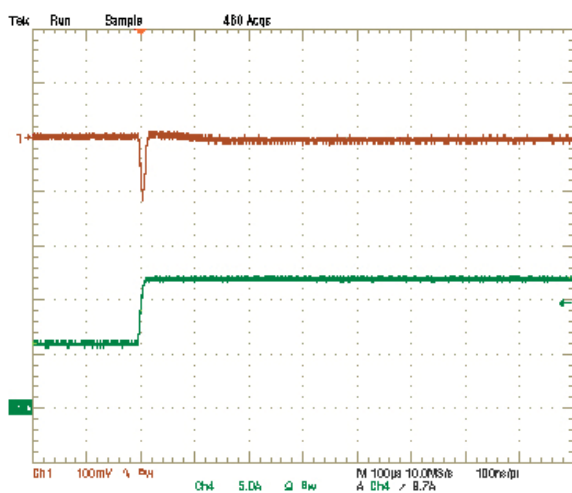
Step Load Transient Response (Vin=5.0V, Vout=3.3V, Cload=94μF, Iout=6A to 12A) Trace 1=Vout, 100 mV/div, Trace 4=Iout, 5A/div.
