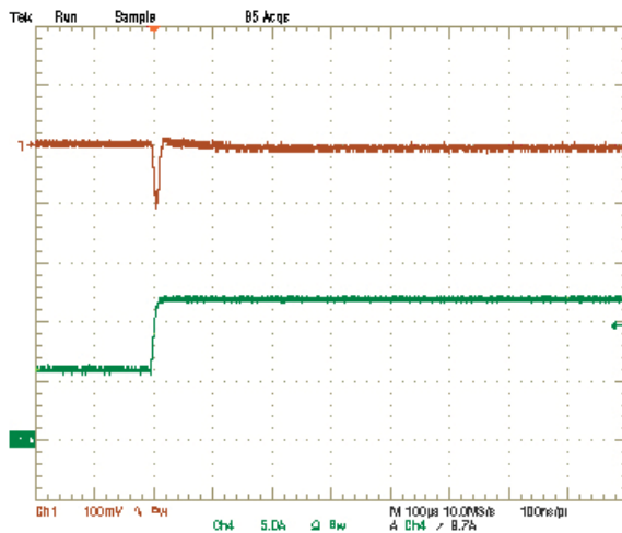
Step Load Transient Response (Vin=5.0V, Vout=2.5V, Cload=94μF, Iout=6A to 12A) Trace 1=Vout, 100 mV/div, Trace 4=Iout, 5A/div.
