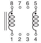
PDLF2000, 2500
