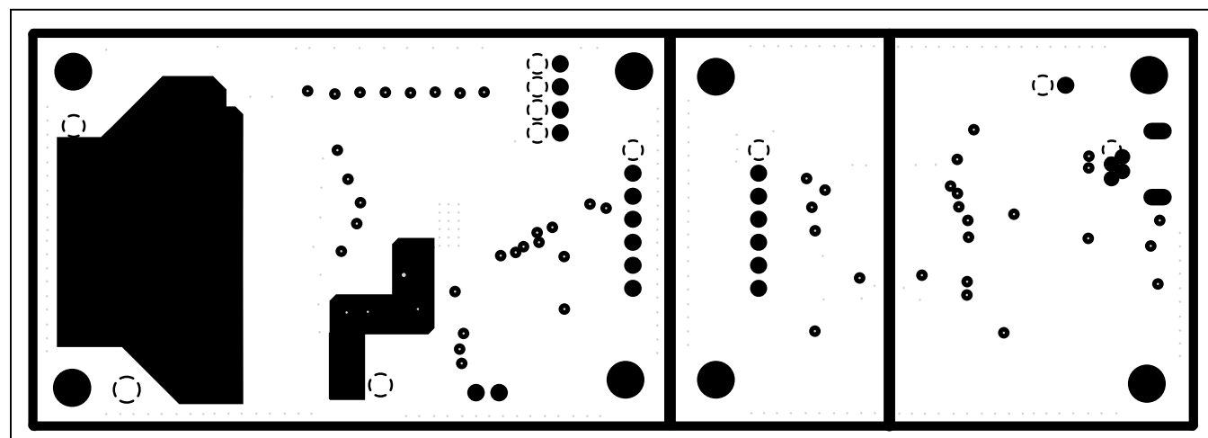
Figure 5. MAX31912/MAX31913 EV Kit PCB Layout—Internal Layer 1
