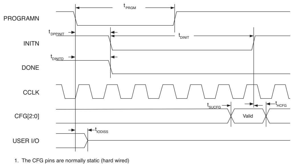
Figure 3-18. Configuration from PROGRAMN Timing
