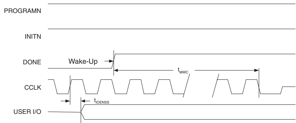
Figure 3-19. Wake-Up Timing
