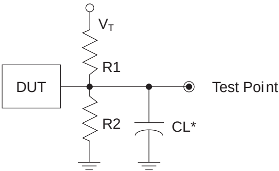
Figure 3-22. Output Test Load, LVTTTL and LVCMOS Standards
