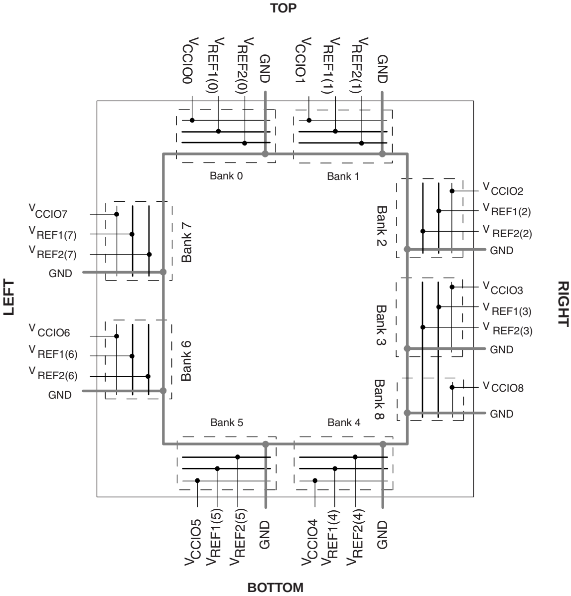
Figure 2-37. LatticeECP2 Banks
