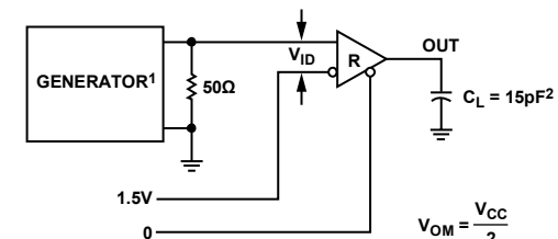
1 PPR = 250kHz, 50% DUTY CYCLE, t_R \leq 6.0ns , Z_O = 50\Omega . 2 C_L INCLUDES PROBE AND STRAY CAPACITANCE.
