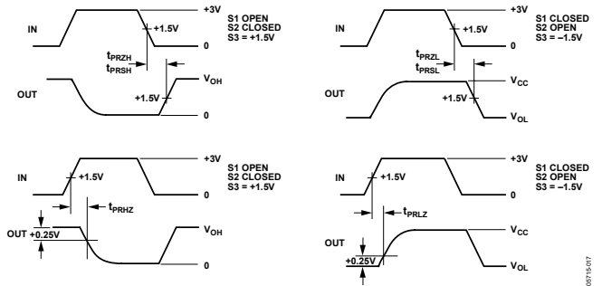
Figure 17. Receiver Enable and Disable Times
