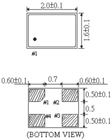
Dimensions: mm
