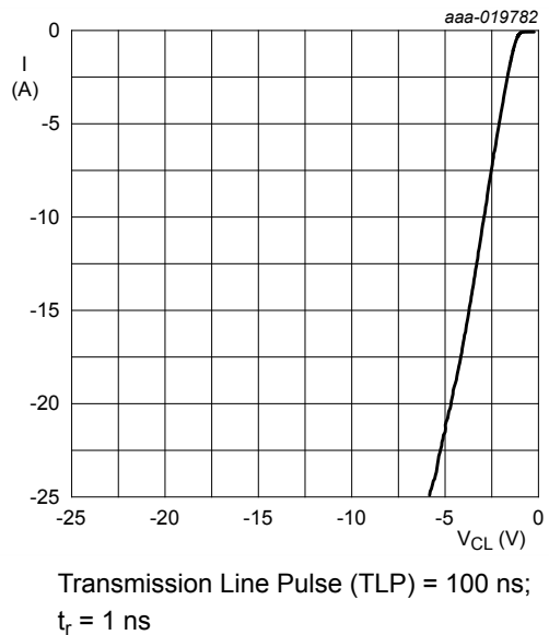
Fig. 18. Dynamic resistance with negative clamping; typical values
