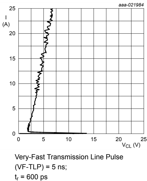
Fig. 19. Dynamic resistance with positive clamping; typical values
