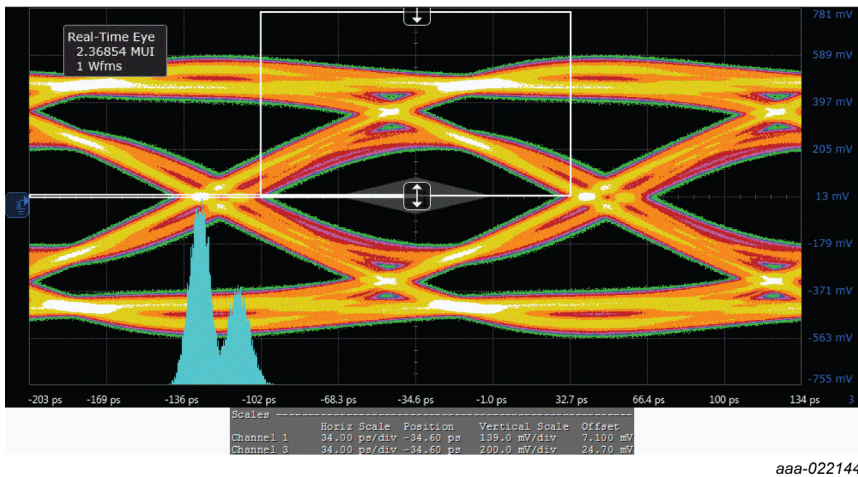
Fig. 11. HDMI 2.0 eye diagram TP2, test board with PCMF2USB3S; typical values
