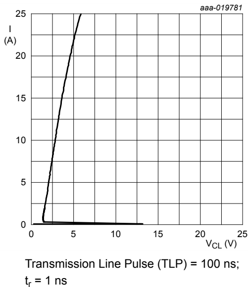
Fig. 17. Dynamic resistance with positive clamping; typical values
