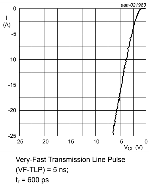
Fig. 20. Dynamic resistance with negative clamping; typical values
