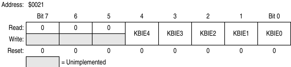
Figure 24-4. Keyboard Interrupt Enable Register (KBIER)
