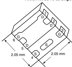
PowerPAK SC-70-6L-Single
