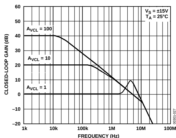
Figure 27. OP482 Closed-Loop Gain vs. Frequency
