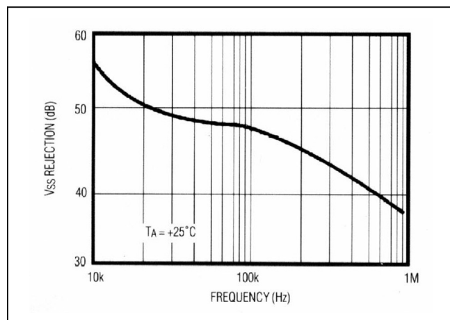
Figure 15. V_{SS} Power-Supply Rejection vs. Frequency
