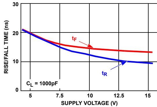
FIGURE 10. RISE/FALL TIME vs SUPPLY VOLTAGE
