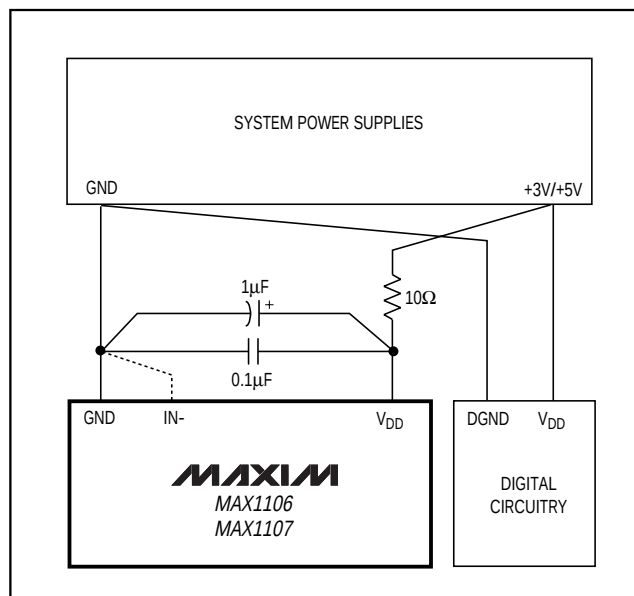
Figure 10. Power-Supply Connections
