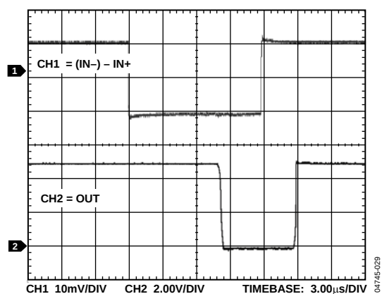
Figure 16. Propagation Delay Timing 10 mV Overdrive
