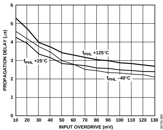
Figure 6. Propagation Delay vs. Input Overdrive (High to Low)
