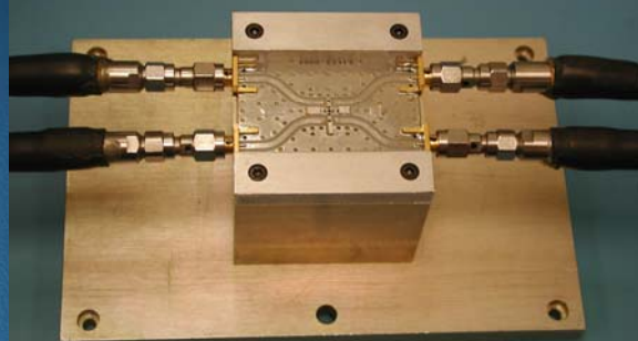
Test Board In Fixture
