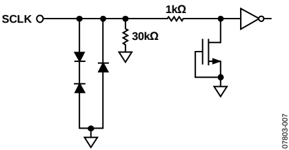
Figure 25. Equivalent SCLK Input Circuit
