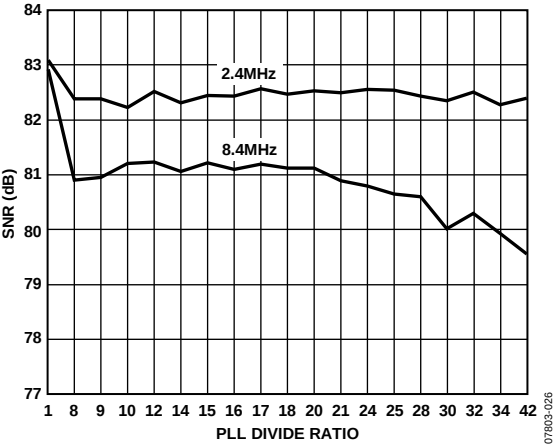
Figure 20. Single-Tone SNR vs. PLL Divide Ratio
