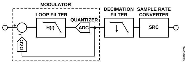
Figure 29. \Sigma - \Delta Modulator Overview
