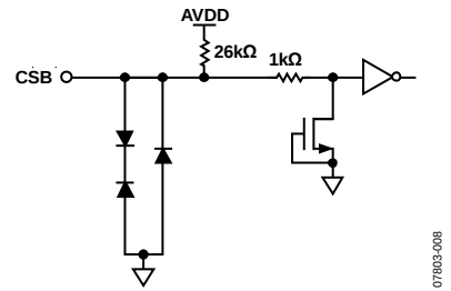
Figure 26. Equivalent CSB Input Circuit
