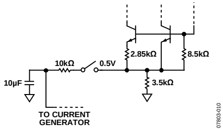
Figure 28. Equivalent VREF Circuit
