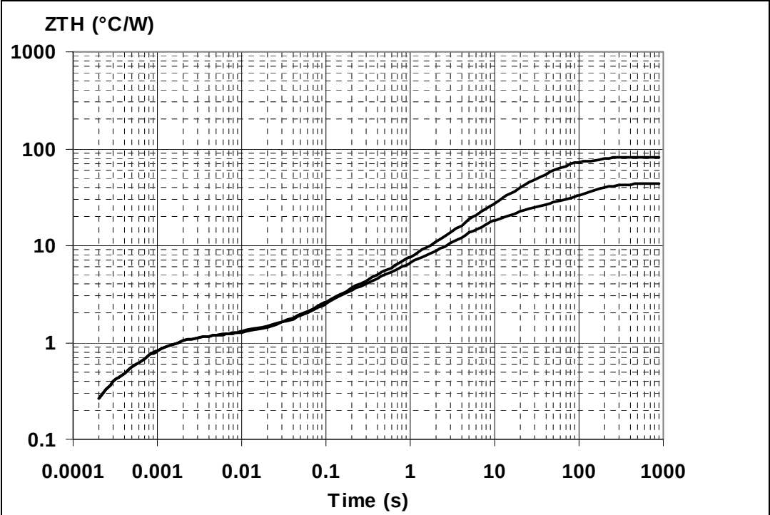
Figure 46. DPAK thermal impedance junction ambient single pulse
