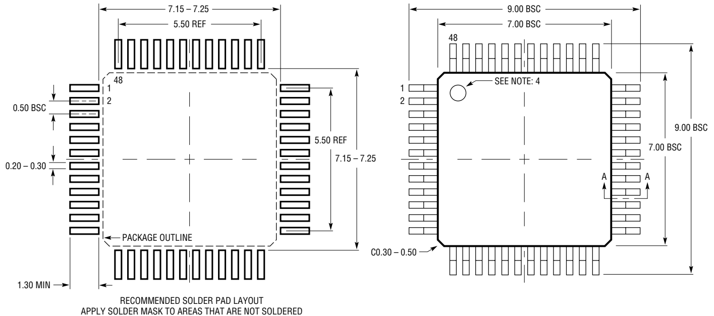
LX Package 48-Lead Plastic LQFP (7mm × 7mm) (Reference LTC DWG # 05-08-1760 Rev 0)
