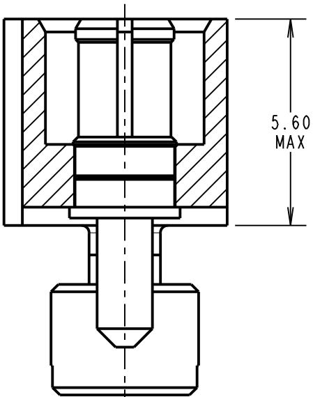
SECTION Z-Z
