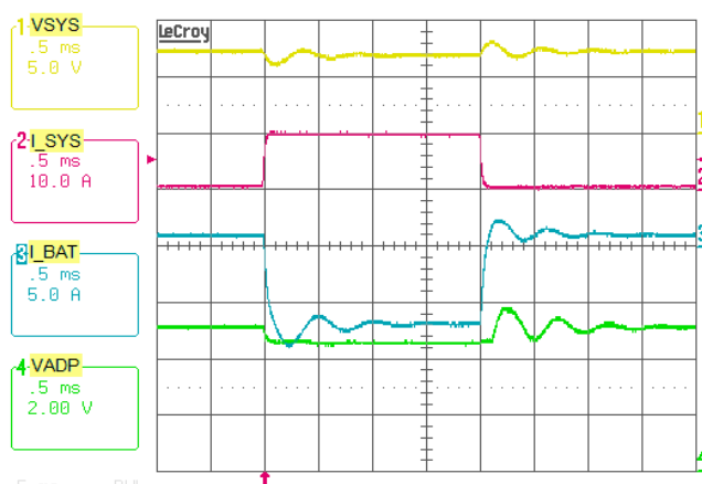
FIGURE 17. BOOST MODE, CHARGING CURRENT LOOP TO INPUT VOLTAGE LOOP TRANSITION. V_{ADP} = 5V , MAXSYSTEMVOLTAGE = 8.496V , V_{BAT} = 7V , VINDAC = 4.5V , SYSTEM LOAD 0.5A TO 10A STEP, CHARGECURRENT = 1A
