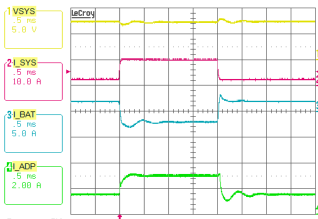
FIGURE 15. BUCK MODE, CHARGING CURRENT LOOP TO ADAPTER CURRENT LOOP TRANSITION. V_{ADP} = 20V , MAXSYSTEMVOLTAGE = 8.496V , V_{BAT} = 7V , SYSTEM LOAD 2A TO 10A STEP, ADAPTERCURRENTLIMIT = 3A , CHARGECURRENT = 2A
