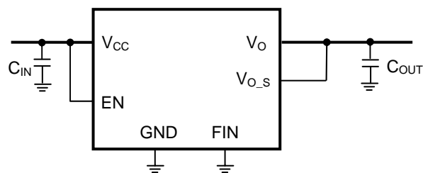
Fixed output voltage type
