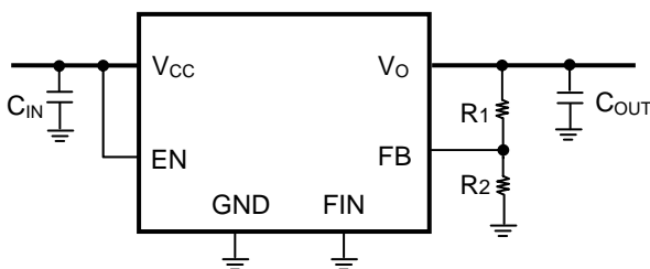
Variable output voltage type
