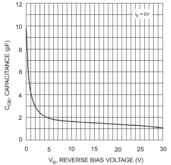
Fig. 4 Output Capacitance
